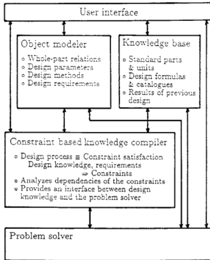
Fig.4 Tool architecture
