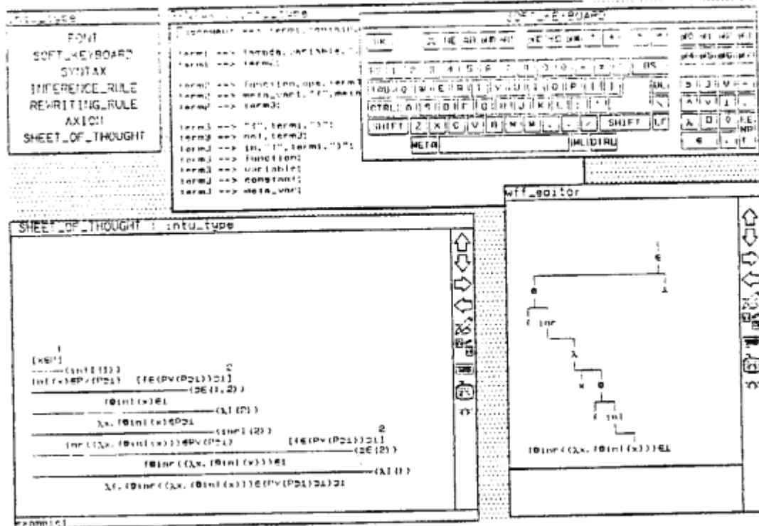
Fig. 1 Reasoning-oriented human-computer interface
