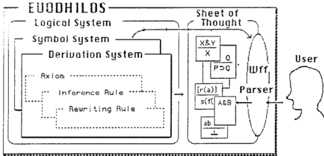
Fig. 2 An illustration of EUODHILOS
