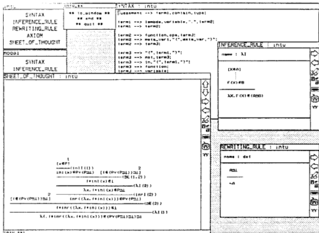
Fig. 3 Screen layout of a constructive proof
