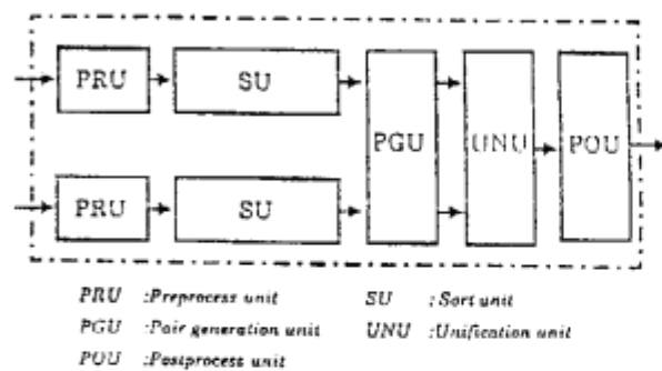
Figure 8. Basic structure of unification engine
