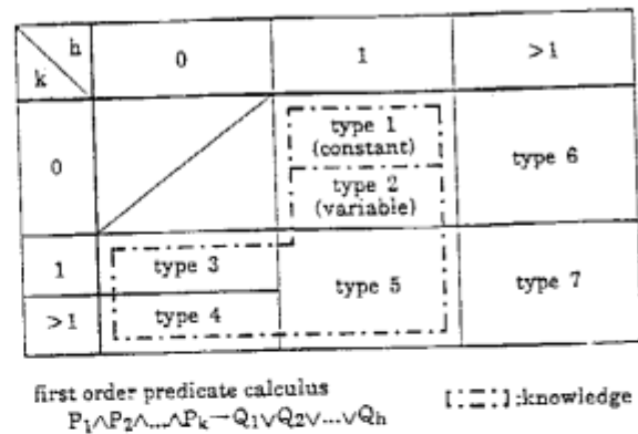
Figure 2. Knowledge representation
