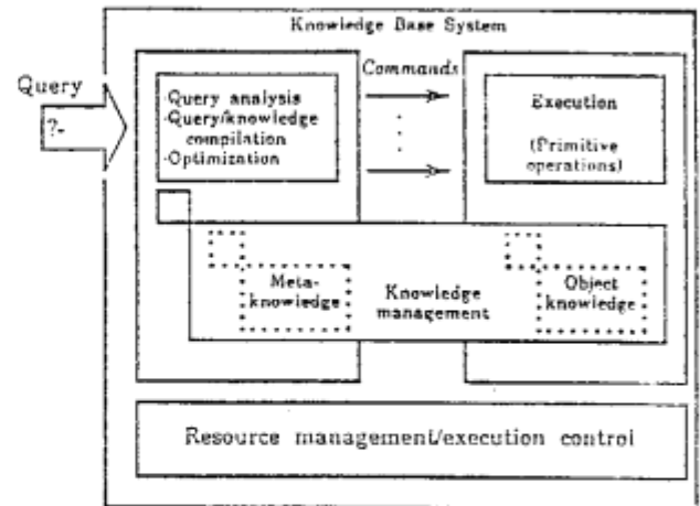
Figure 5. Optimization strategy using meta-knowledge position of the query
