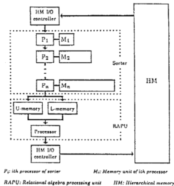
Figure 7. Hardware configuration of relational engine
