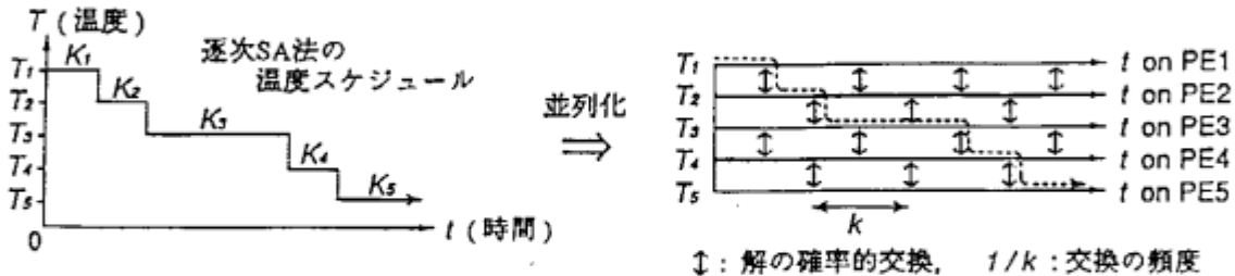
図 1: Temperature Parallel Simulated Annealing
