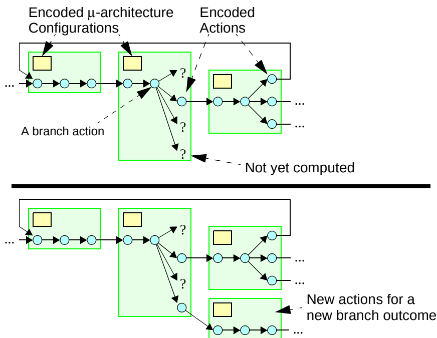
図 4 fast-forwarding [5]
